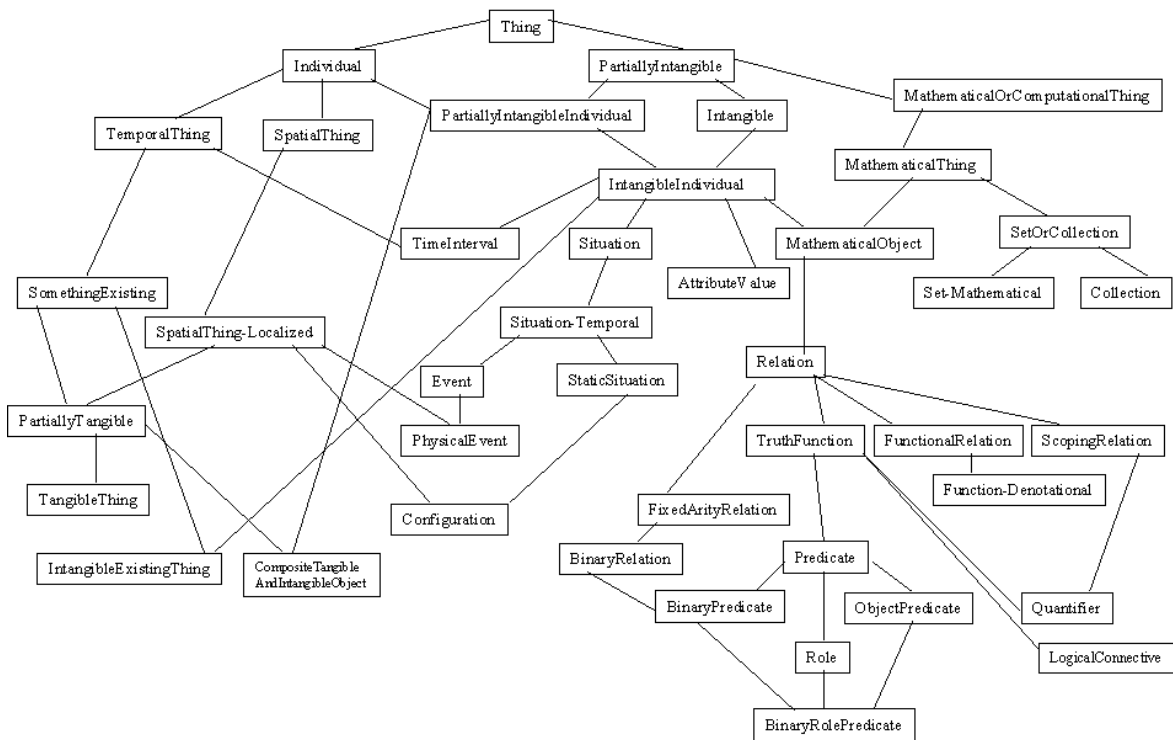
Fig. 6 Upper ontology of OpenCyc http://www.cyc.com/cycdoc/vocab/upperont-diagram.html
