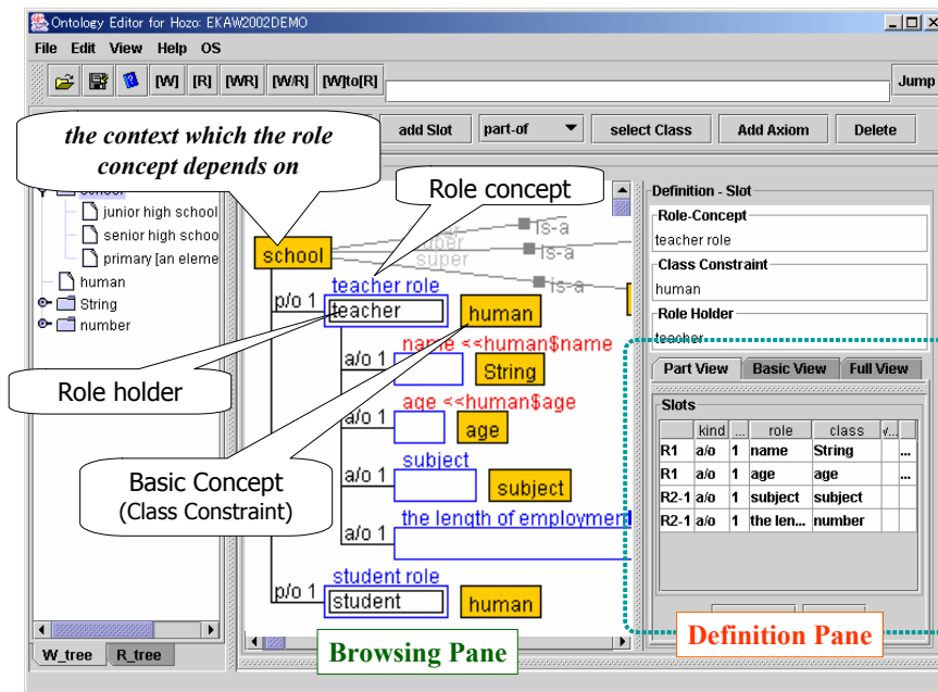
Fig. 4 GUI of Ontology Editor in Hozo.
